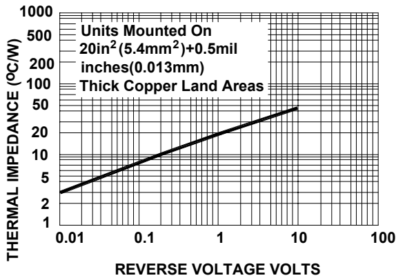
Fig. 5-TRANSIENT THERMAL IMPEDANCE
