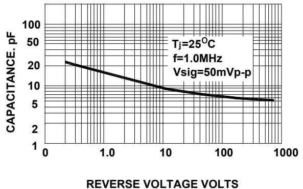
Fig. 6-TYPICAL JUNCTION CAPACITANCE
